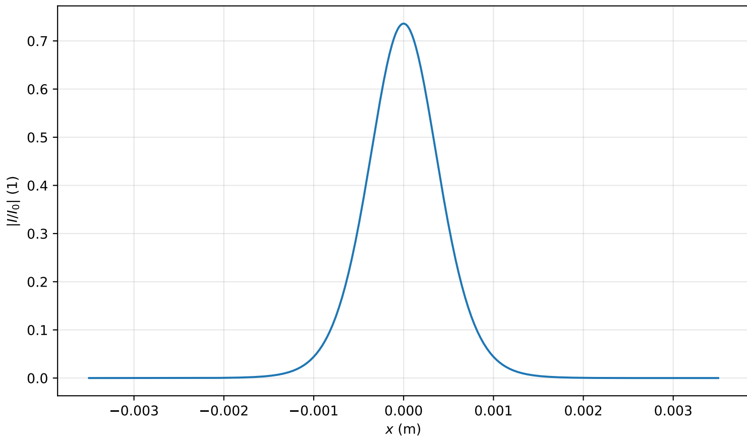
Intensity profile I(x, y = 0, z = 2.309m)/I_0 , P_{in}=0.5P_{cr} , artificial time
